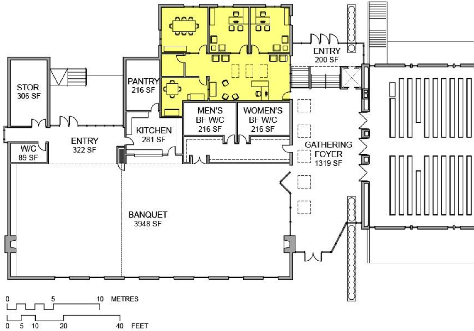
Main Floor Plan – Administration Area
