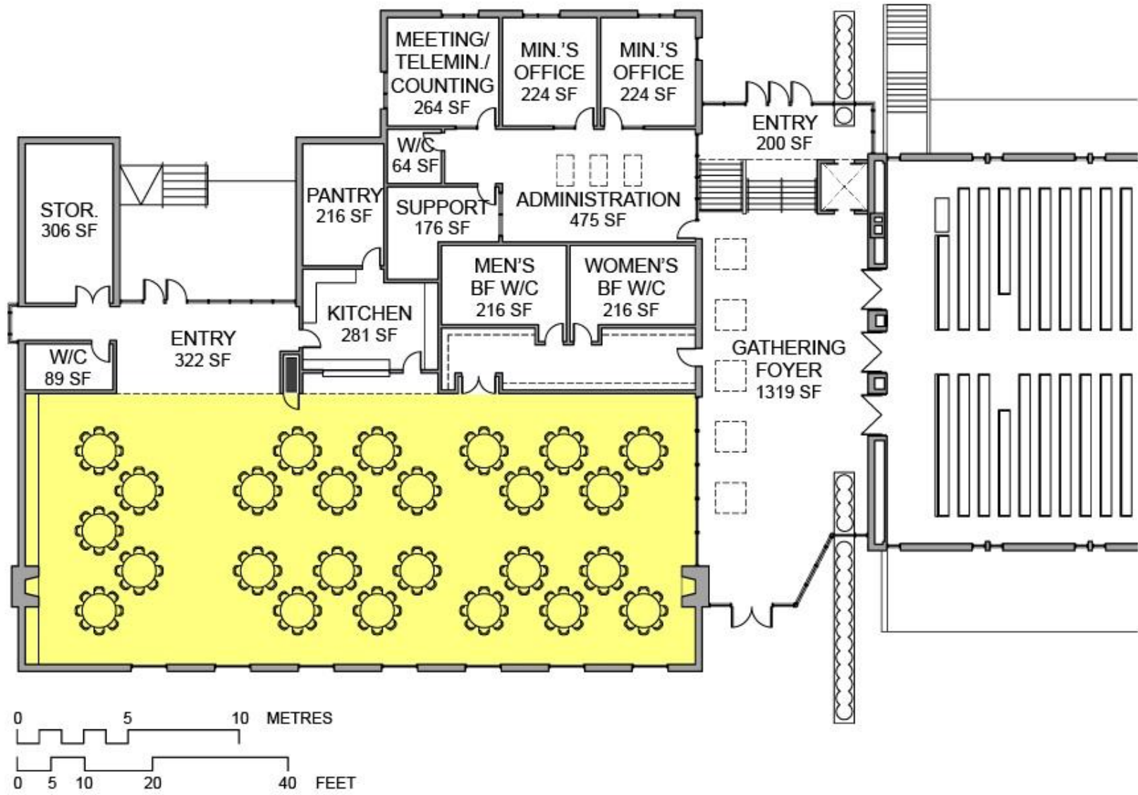
Main Floor Plan – Banquet for 200 Persons
