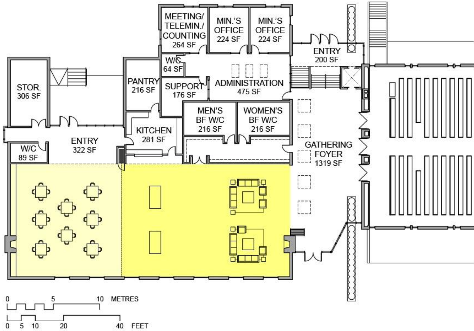
Main Floor Plan – Small Banquet & Informal Seating
